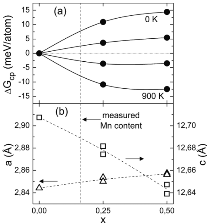
FIG. 1. (a) \Delta G_{cp} = \Delta H_{cp} - TS for (Cr_{1-x}Mn_x)_2AlC from 0 to 900 K, in steps of 300 K. (b) Lattice parameters a and c for (Cr_{1-x}Mn_x)_2AlC for two different SQS supercells. The curves act as a guide for the eye, and represent average values of the two supercells.
