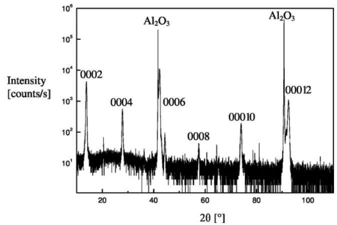
FIG. 2. \theta - 2\theta XRD scan from a (Cr_{1-x}Mn_x)_2AlC film deposited on Al_2O_3(0001) . An extra peak at 44.4^\circ originates from CrMn.
