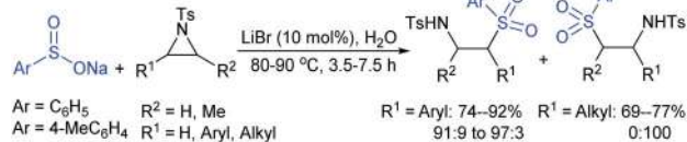
Scheme 252 LiBr catalyzed the regioselective sulfonylation of aziridines with sodium sulfonates.
