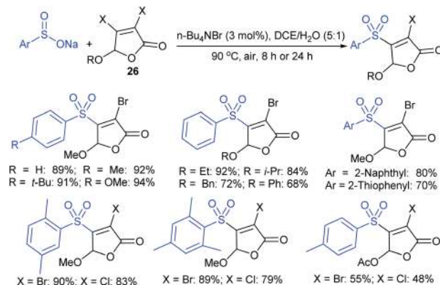
Scheme 86 TBAB-catalyzed sulfenylation of 3,4-dihalo-5-alkoxy-2(5 H )-furanones with sodium sulfinates.
