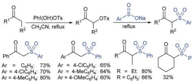
Scheme 138 \alpha -Tosyloxylation of ketones with HTIB and sulfonylation using sodium sulfonates.
