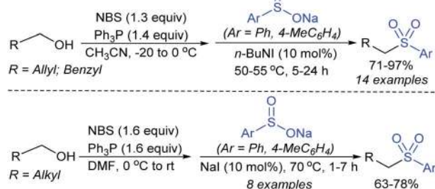
Scheme 254 One-pot bromination-sulfonylation of primary alcohols with sodium arenesulfonates.
