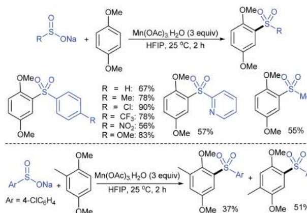
Scheme 193 Mn(OAc) 3 -promoted oxidative C-H sulfonation of 1,4-dimethoxybenzene with sodium sulfonates.
