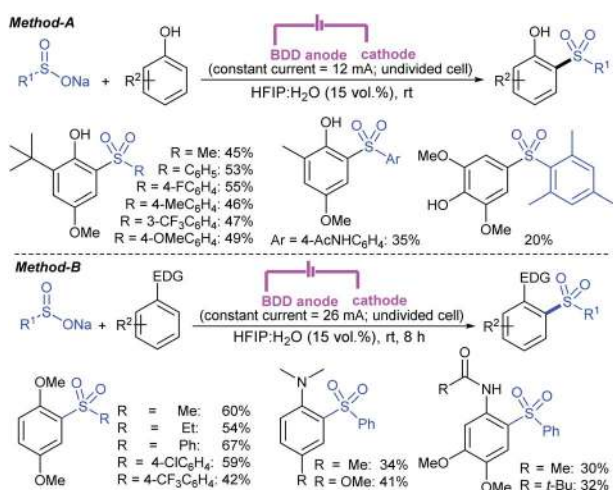
Scheme 191 Electrochemical sulfonation of arenes and aniline derivatives with sodium sulfonates.
