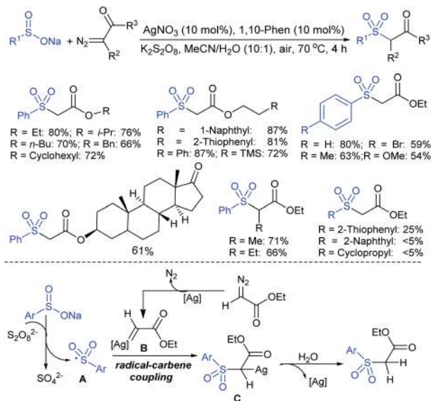
Scheme 153 AgNO_3 -catalyzed radical-carbene coupling of \alpha -diazo carbonyl compounds with sodium sulfonates and the proposed reaction mechanism.
