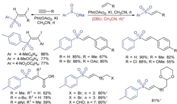
Scheme 88 \text{PhI}(\text{OAc})_2 -mediated sulfonylation of alkenes and alkynes with sulfonates.
