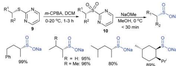
Scheme 9 Synthesis of optically pure sodium sulfinate salts.
