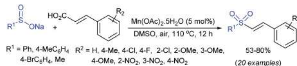
Scheme 118 Decarboxylative coupling of cinnamic acids with sulfinate salts.
