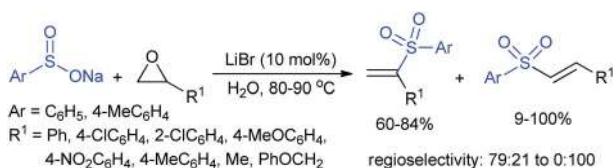
Scheme 78 Synthesis of vinyl sulfones via the opening of epoxides with sodium sulfonates.
