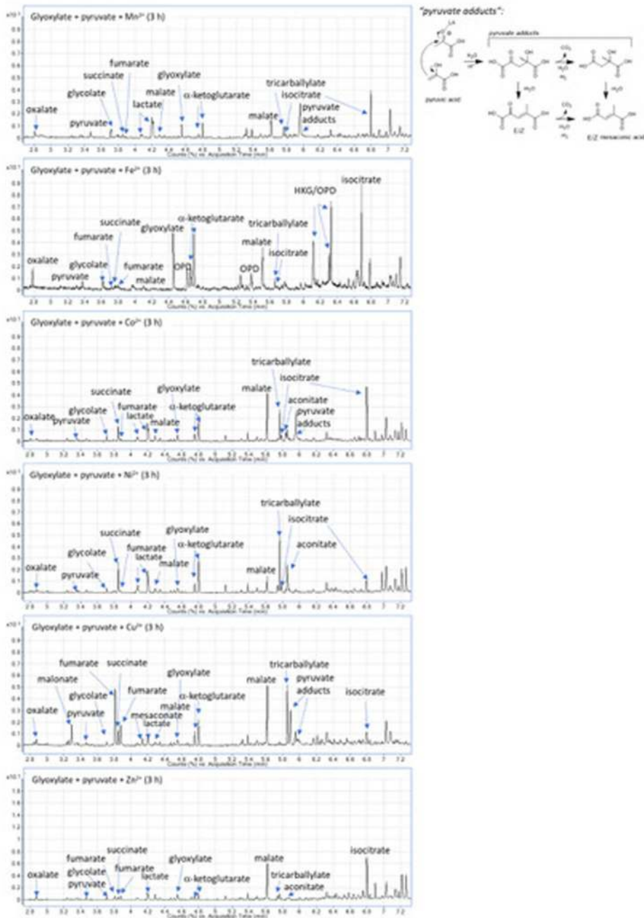
Extended Data Figure 1. Transition metal screen. GC chromatograms showing a reaction network arising from pyruvate and glyoxylate, promoted by transition metal ions at 70 °C (qualitative screen).
