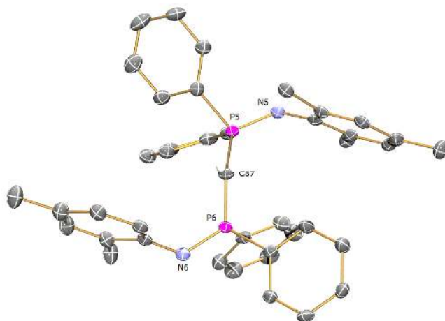
Figure 6. Anionic component of 5a 4C_7H_8 . Displacement ellipsoids are drawn at 50% probability, with lattice solvent and non-methanide hydrogen atoms omitted for clarity.
