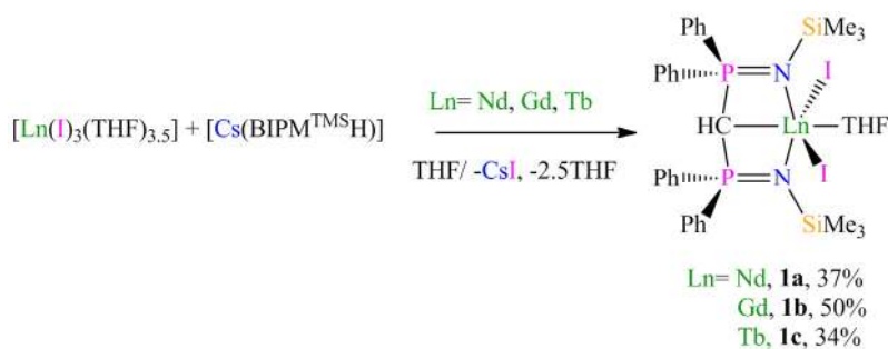
Scheme 1. Preparation of 1a–c .
