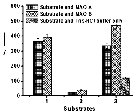
Figure 3. Fluorescence enhancement of MAO-HPQ substrates: 1–3 ( 200 \mu\text{M} ) in 100 \text{ mM} of Tris-HCl buffer, pH 7.90 incubated with enzymes ( 10 \mu\text{g mL}^{-1} ) for 2 h.
