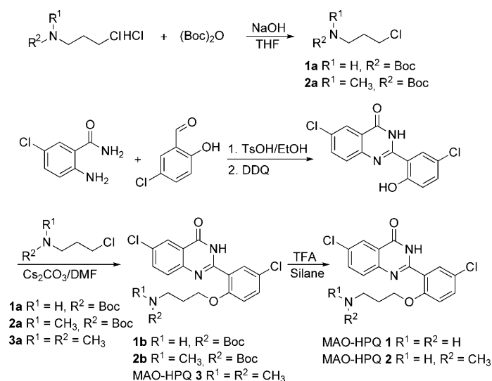
Scheme 2. Synthetic route for fluorogenic probes MAO-HPQ 1–3.
