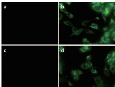
Figure 5. Representative fluorescence images of C6 glioma cells and PC12 cells with MAO-HPQ 1 (100 \mu\text{M} ) and inhibitors (100 \mu\text{M} ) incubated separately at 37 ^{\circ}\text{C} with 5% \text{CO}_2 for 60 min. Excitation filter: 360/40 nm; emission filter: 535/40 nm. a) C6 glioma cells incubated with MAO-HPQ 1 ; b) PC12 cells incubated with MAO-HPQ 1 ; c) clorgyline pretreated PC12 cells incubated with MAO-HPQ 1 ; d) pargyline pretreated PC12 cells incubated with MAO-HPQ 1 .
