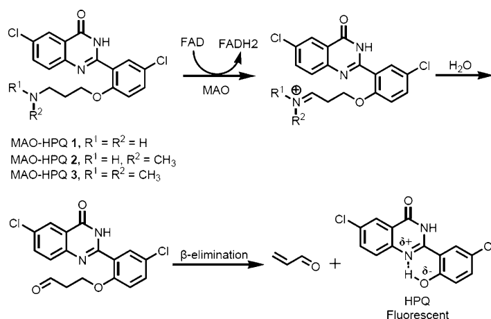
Scheme 1. Fluorescence detection of MAO activity by oxidative deamination of HPQ derivatives and subsequent \beta -elimination.
