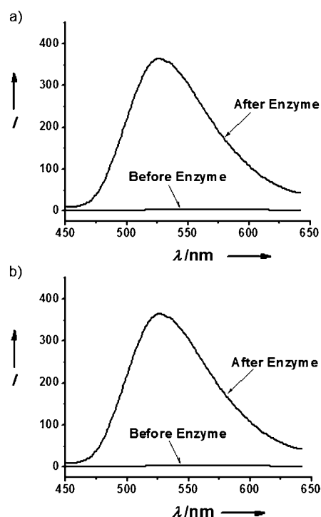
Figure 1. Fluorescence measurement of MAO enzymatic reactions. Emission spectrum of MAO-HPQ 1 (200 μM) upon treatment with MAO A (a) and MAO B (b) in Tris-HCl buffer (100 mM, pH 7.90). Enzyme concentration: 10 μg mL -1 . Excitation wavelength: 360 nm; emission wavelength: 530 nm.
