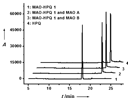
Figure 2. HPLC analysis of enzymatic reaction of MAO-HPQ 1 with MAO isozymes. Absorbance wavelength: 360 nm
