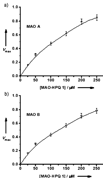
Figure 4. Enzymatic kinetics of MAO activity with MAO-HPQ 1 . Data show the relative reaction rates over a range of concentrations of substrate. These values were obtained from an average of at least six independent experiments for each concentration and were collected over a time frame of 60 min. The reactions were performed at 37^\circ\text{C} in Tris-HCl Buffer at pH 7.90. These readings were collected at a final enzyme concentration of 5 \mu\text{g mL}^{-1} . Excitation wavelength: 360 nm; emission wavelength: 530 nm.
