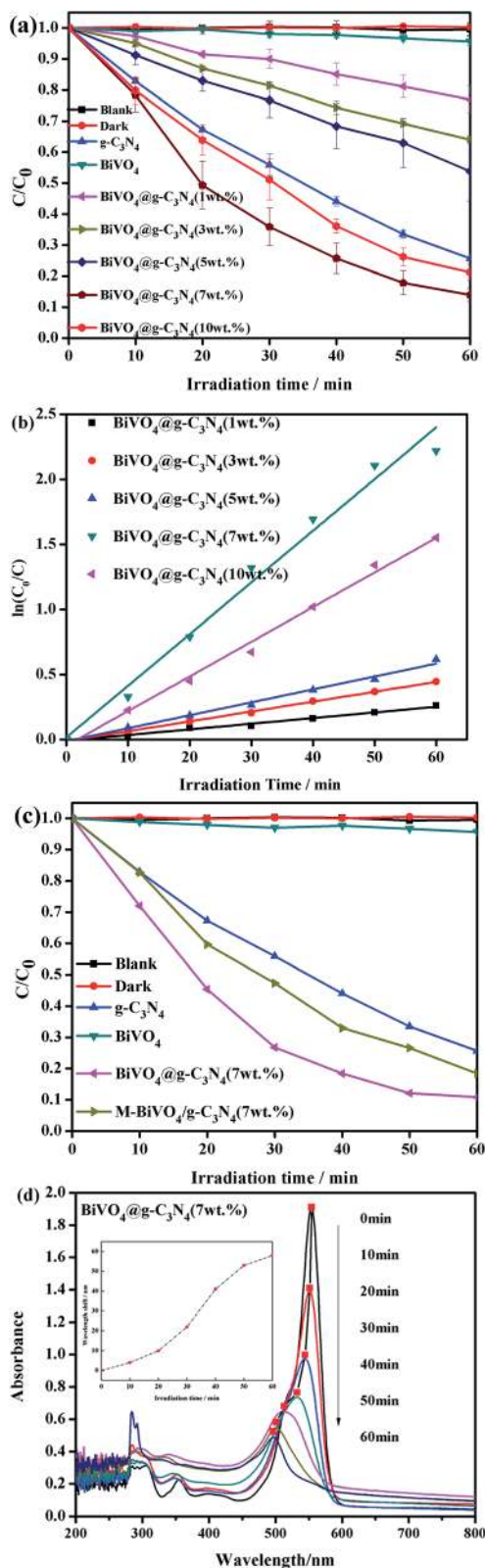
Fig. 8 (a) The comparison of photocatalytic activity for g\text{-C}_3\text{N}_4 , \text{BiVO}_4 and \text{BiVO}_4@g\text{-C}_3\text{N}_4 ( x wt%) ( x = 1, 3, 5, 7, 10 ); (b) the comparison of first-order kinetic constants of different photo-catalysts; (c) the comparison of photocatalytic activity for \text{BiVO}_4@g\text{-C}_3\text{N}_4 (7 wt%) and \text{M-BiVO}_4/g\text{-C}_3\text{N}_4 (7 wt%); (d) the whole spectral scanning of RhB during the photo-catalytic degradation for \text{BiVO}_4@g\text{-C}_3\text{N}_4 (7 wt%).
