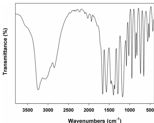
Fig. 3. FTIR spectrum of ammonium acesulfamate in the spectral range between 4000 and 400 \text{cm}^{-1} .
