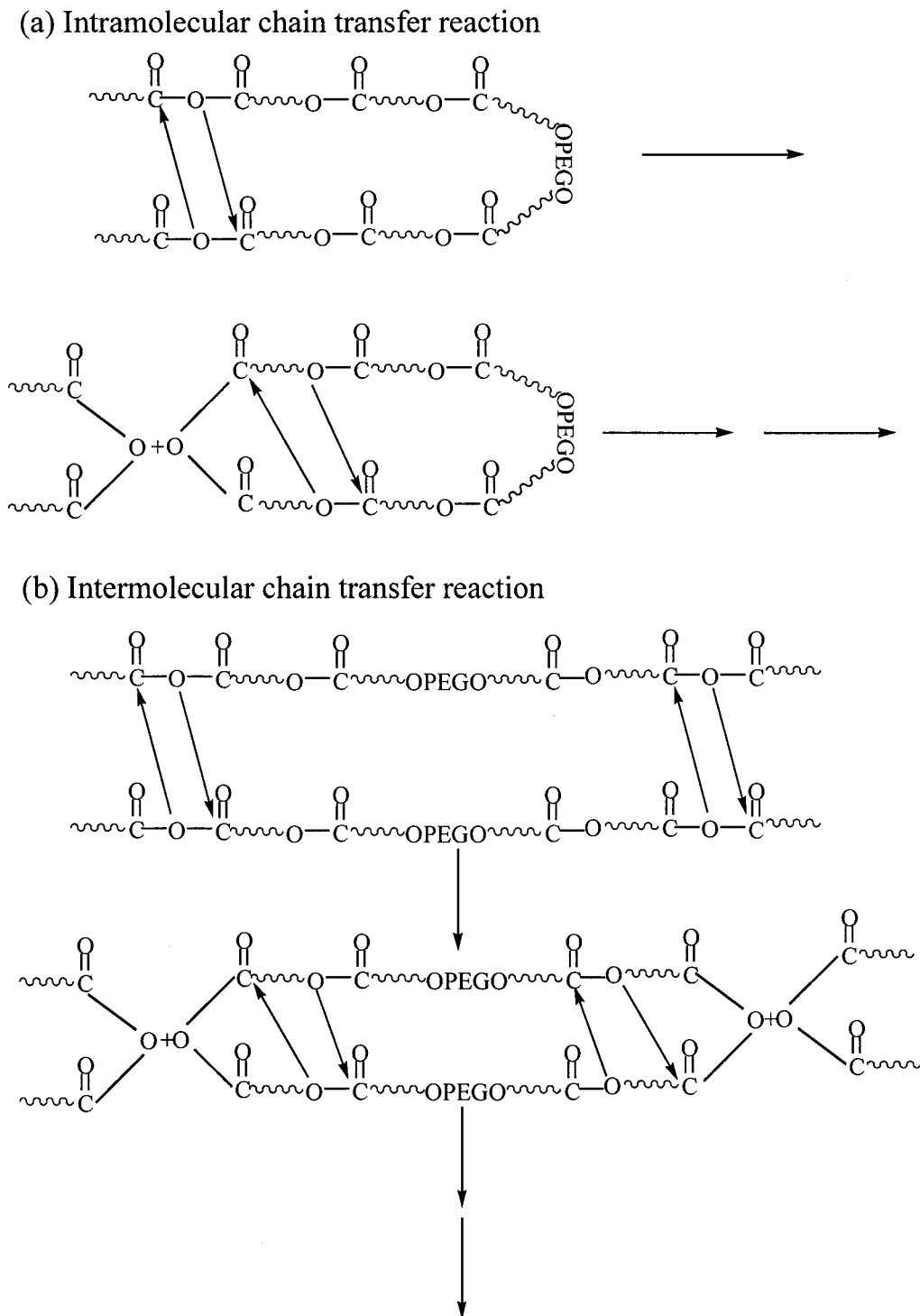
Scheme 2. Possible mechanism of chain-transfer reactions.
