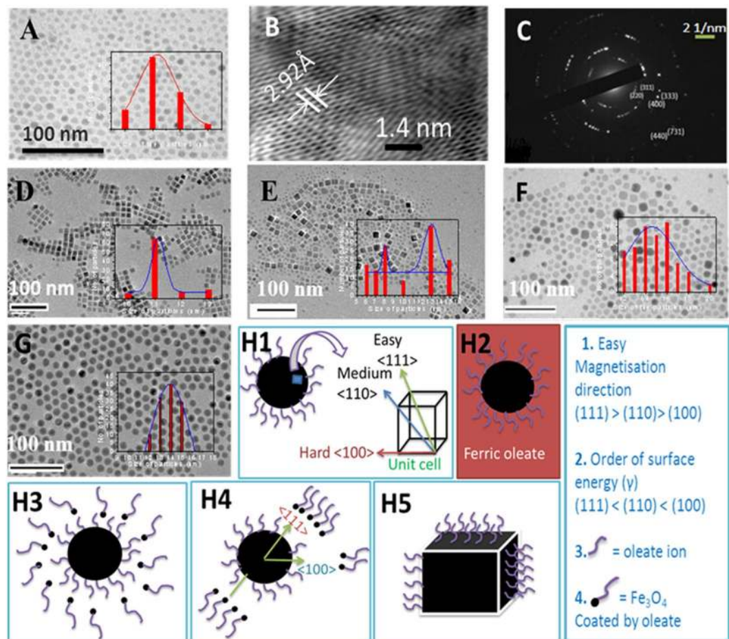
Figure 2. Core Fe 3 O 4 particles (heating rate of 4 °C per minute): (A) TEM image, (B) HRTEM image, (C) SAED pattern. Core-shell Fe 3 O 4 @Fe 3 O 4 particles after addition of (D) 1 mL and (E) 5 mL of ferric oleate (duration of heating is 1 hour) and (F) 5 mL of ferric oleate (duration of heating is 8 hour). (G) core Fe 3 O 4 particles prepared by heating rate of 1.3 °C/min. Schematic diagram of conversion of spherical to cubic shape of a particle by core-shell model (Ostwald ripening phenomenon): (H1) slightly spherical particle coated by oleate ions along with magnetisation axes of face-centred cube (Fe 3 O 4 unit cell), (H2) particles in ferric oleate medium, (H3) formation of Fe 3 O 4 small particles/cluster which surrounds a larger particle, (H4) Faster growth/ deposition along <111> direction as compared to <100> or <220> direction, (H5) formation of cubic shaped particle.
