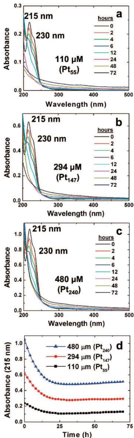
Figure 1. Time-resolved UV-vis spectra showing the hydrolysis of \text{K}_2\text{PtCl}_4 at concentrations of (a) 110, (b) 294, and (c) 480 \mu\text{M} , which represent the concentrations used for the synthesis of \text{G6-OH}(\text{Pt}_n) , n = 55, 147, and 240, DENs, respectively. (d) Plots of the absorbance at \lambda = 215 nm (from parts a–c) as a function of time for the data shown in parts a–c. The reduction in the intensity of this peak corresponds to hydrolysis of \text{PtCl}_4^{2-} .
