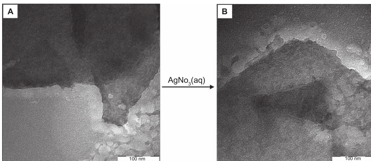
Figure 3 Transmission electron microscopy images of (A) pure talc and (B) talc after impregnation with aqueous \text{AgNO}_3 ( \text{AgNO}_3 /talc, A0).
