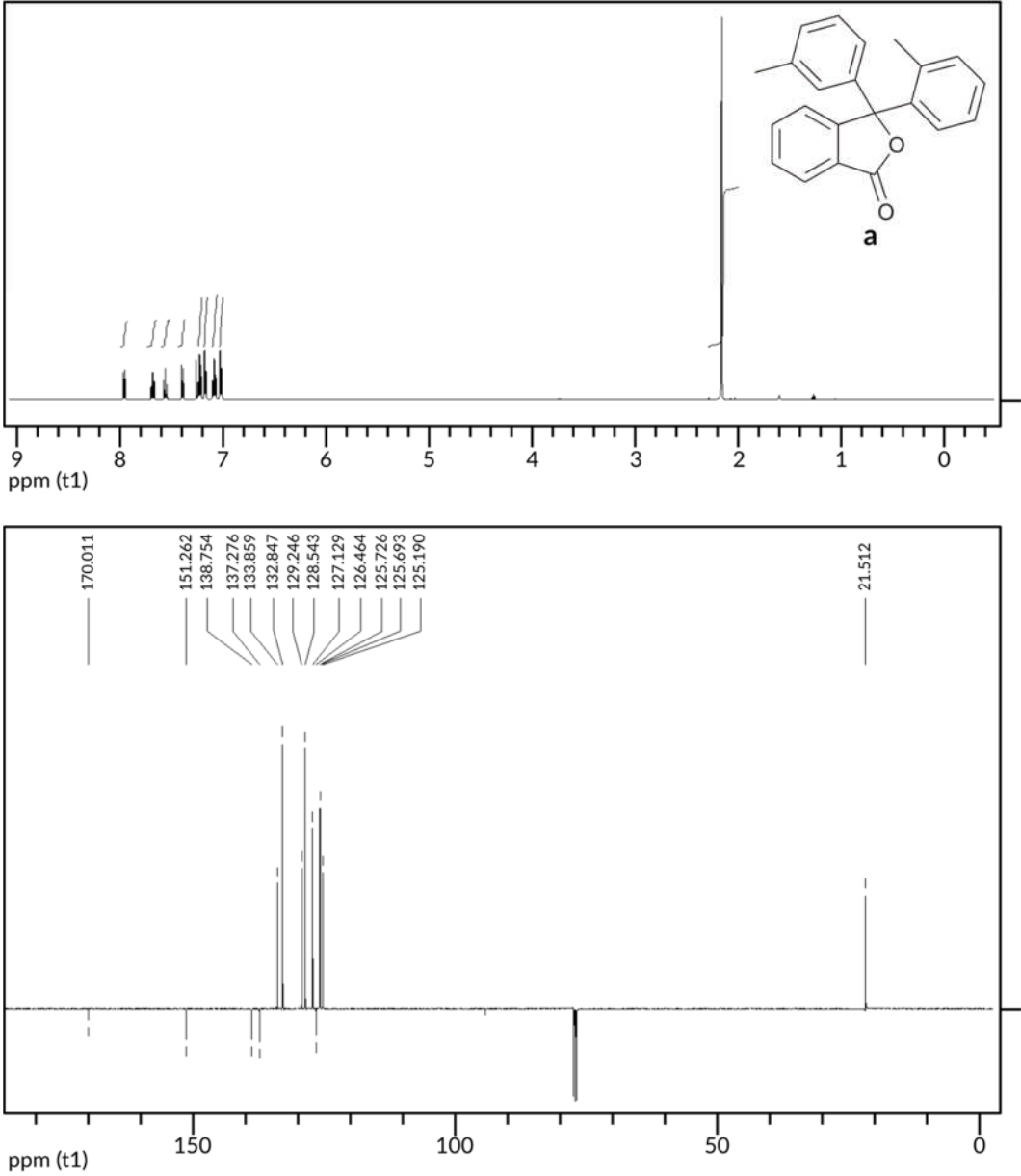
1 H (top) and 13 C (bottom) NMR spectra of compound a .
