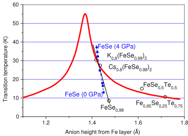
Figure 4. Dependence of T_c on the distance between Fe and the chalcogenide/pnictide layers. The red line shows the dependence as presented by Mizuguchi et al [17] for typical Fe-based superconductors. The filled circles indicate the data obtained for FeSe under high pressure [2]. The open points indicate the data obtained by this work and our previous reports [18, 19].
