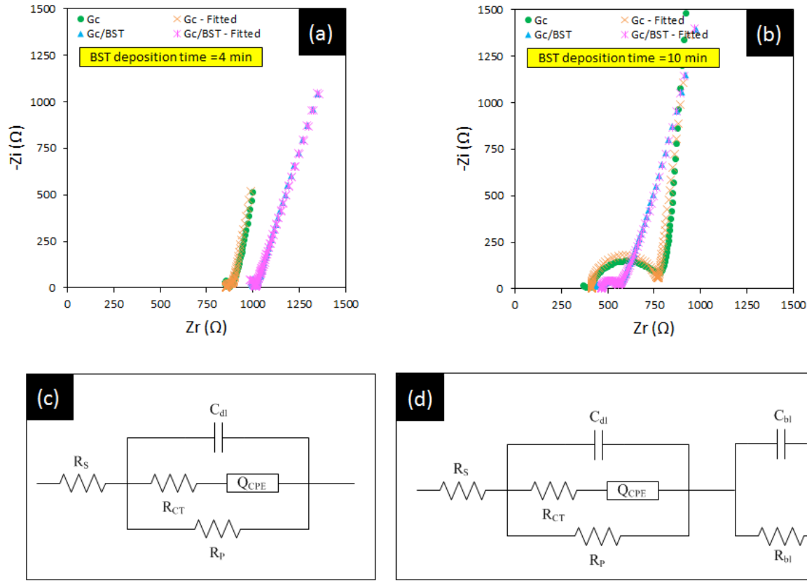
Figure 4.9 (a) and (b) measured and fitted EIS of G_c and G_c/BST_c at different deposition times. (c) circuit model used to fit G_c , and (d) circuit mode used to fit G_c/BST_c .
