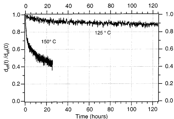
Figure 3. Temporal stability of AC2729 at 125 and 150 °C.
