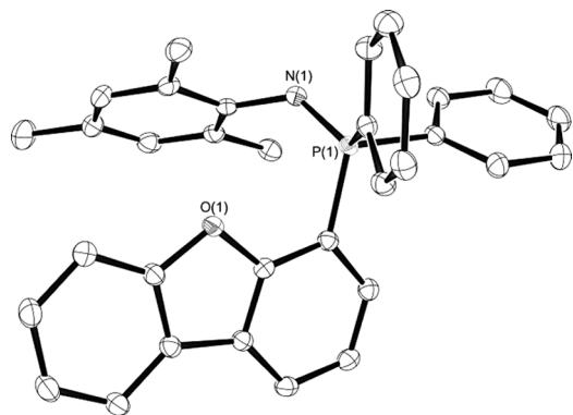
Figure 1. Thermal ellipsoid plot of one of two crystallographically unique molecules of L^{\text{Mes}} in the crystal lattice, with hydrogen-atoms and a molecule of toluene omitted for clarity. Thermal ellipsoids are drawn at the 30% probability level.
