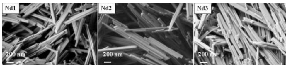
FIG. 5. SEM images of NdPO 4 synthesized at several conditions ( °C/ \tau , h): 1 – 200/55, 2 – 200/100, 3 – 160/100
