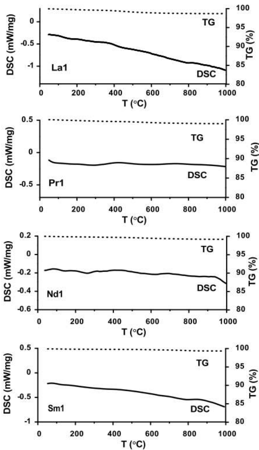
FIG. 2. DSC/TG plots of \text{LnPO}_4 ( \text{Ln} = \text{La}, \text{Pr}, \text{Nd}, \text{Sm} ) synthesized at 200^\circ\text{C}/55\text{ h}
