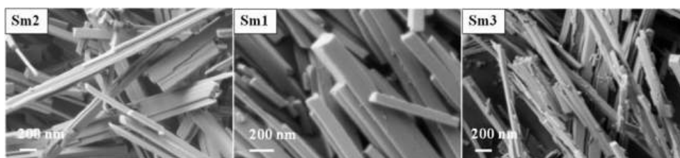
FIG. 6. SEM images of \text{SmPO}_4 synthesized at several conditions ( ^{\circ}\text{C}/\tau , h): 1 – 200/55, 2 – 200/100, 3 – 160/100
