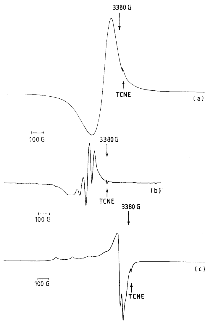
Figure 1. EPR spectra of Cu(AcPA) 2 complex in solid at (a) 300 K, DMSO (b) 300 K and (c) 77 K.
