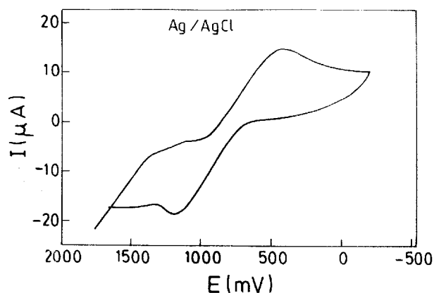
Figure 2. Cyclic voltammogram of Cu(AcPA) 2 at 300 K in DMSO solution; Scan rate 100 mVs -1 .
