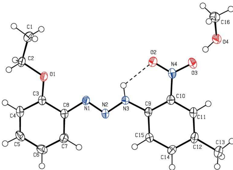
Figure 4. Molecular structure of compound (4) with thermal ellipsoids drawn at 50% probability level. The intramolecular N3\text{--}H3A \cdots O2 hydrogen bond is shown as dashed line.
