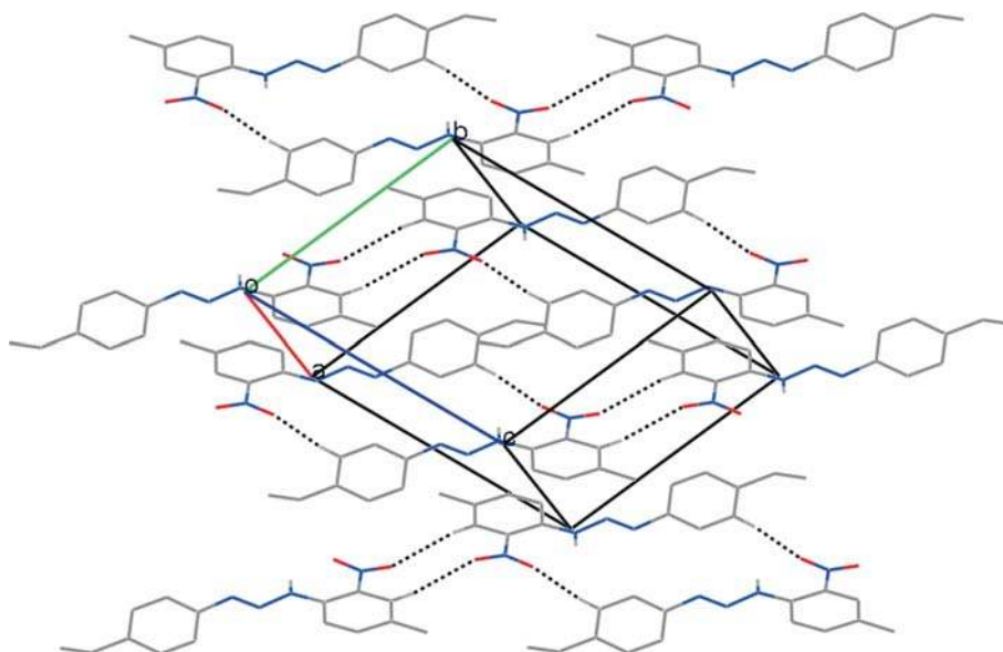
Figure 3. Non-classic C4\text{--}H4 \cdots O1 and C11\text{--}H11 \cdots O2 hydrogen bonds connect the triazene molecules (3) into chains along [110] direction.
