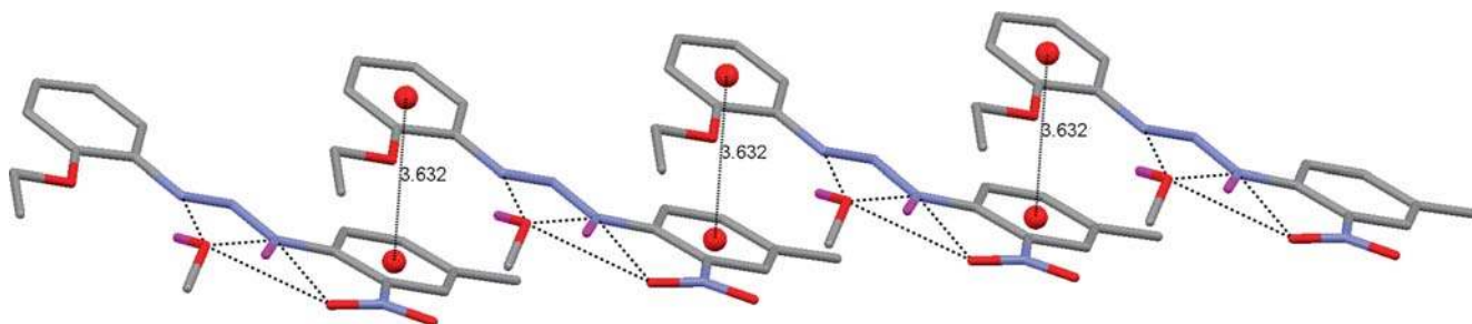
Figure 5. \pi \cdots \pi stacking interactions between Cg1 \cdots Cg2 with centroid-centroid distances of 3.632 (15) Å in compound (4). All hydrogen bonds are also shown as dashed lines. Methanol molecule makes two distinct hydrogen bonds with triazene (4).
