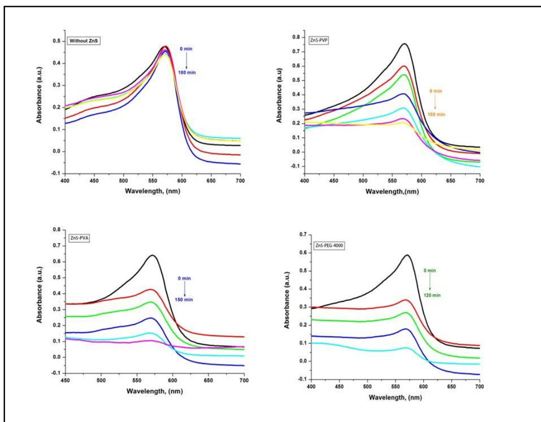
Fig. 5 The absorption spectrum of 0.038gr/LXO solution only (a) and photodegradation of XO dye solution by (b) PVP, (c) PVA and (d) PEG-4000 capped ZnS nanoparticles under sunlight irradiation.
