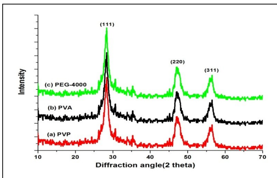
Fig. 2 XRD pattern of ZnS nanoparticles with various capping agents.
