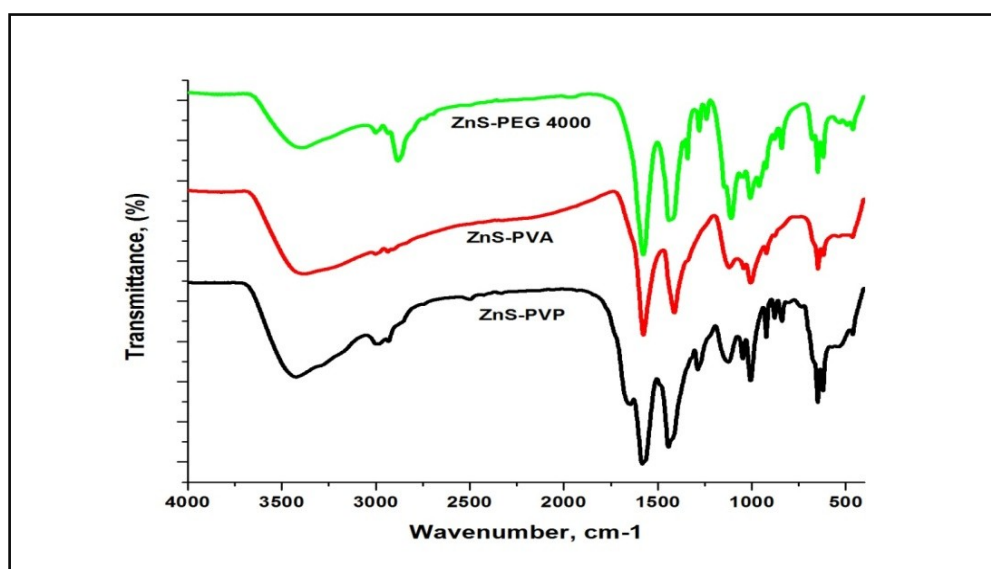
Fig. 3 FTIR spectrum of ZnS nanoparticles with various capping agents.
