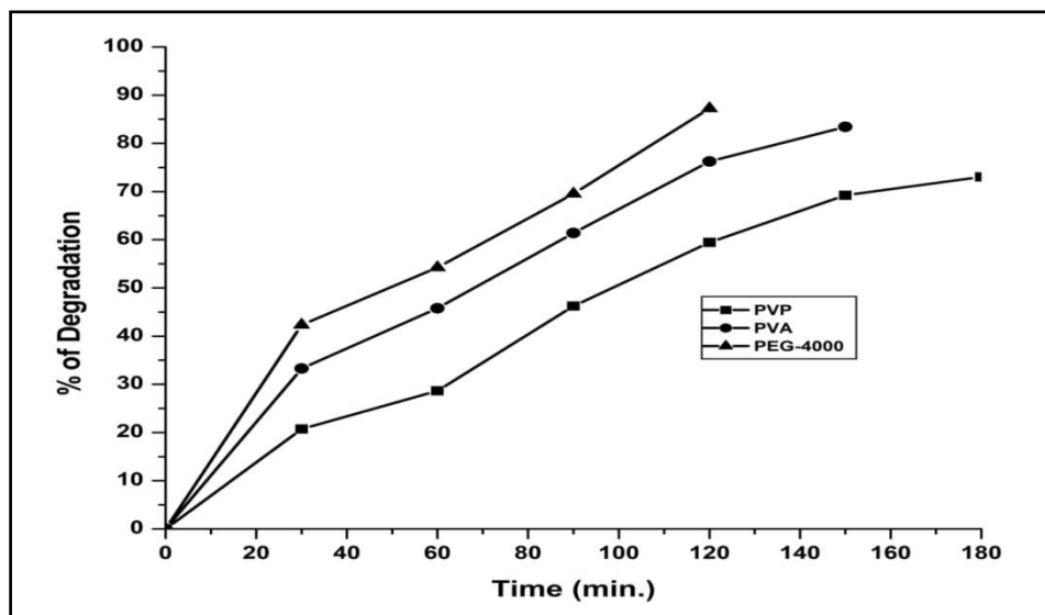
Fig. 6 The effect of XO dye degradation by various capping agents capped ZnS nanoparticles.
