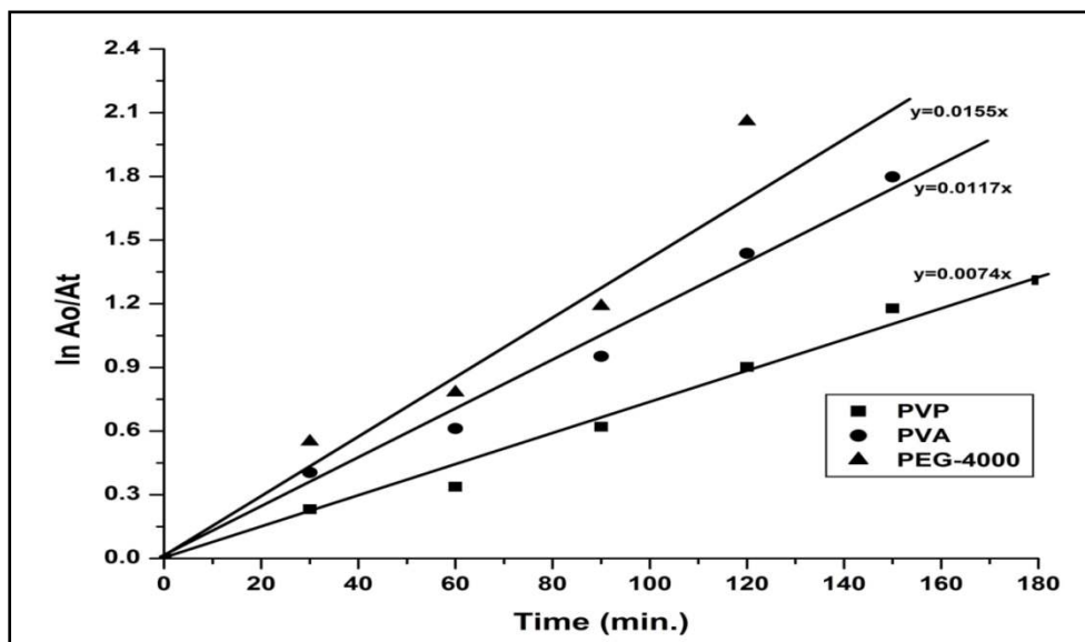
Fig. 7 Kinetic study of photo degradation of XO in the presence of ZnS nanoparticles.
