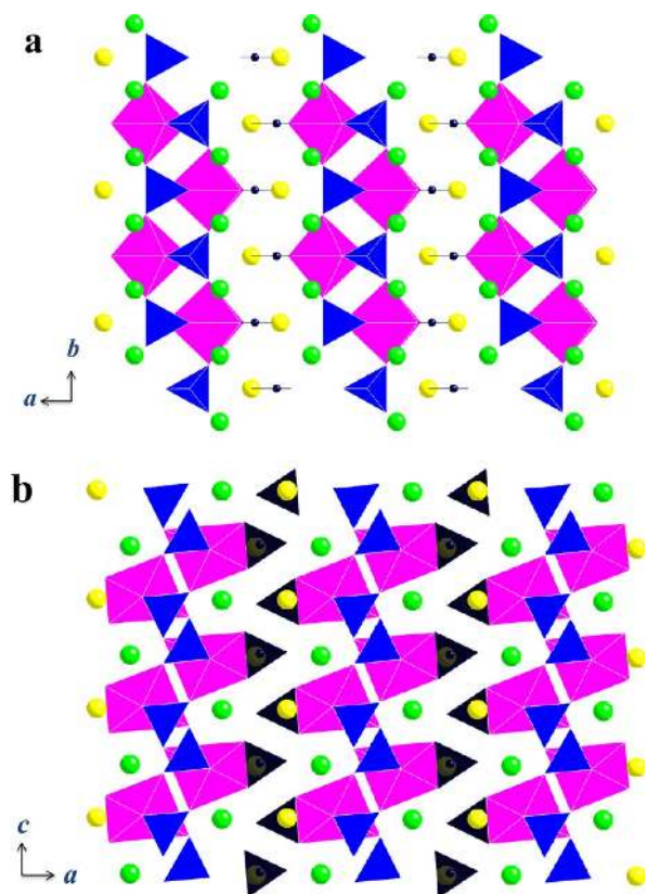
Figure 2. Structure of \text{Na}_3\text{MPO}_4\text{CO}_3 ( M = \text{Mn, Fe, etc.} ) viewed from [001] (a) and [010] (b). Transition metal octahedra, purple; \text{PO}_4 tetrahedra, blue; \text{CO}_3 triangle planar, black; Na, green (Na1) and yellow balls (Na2).
