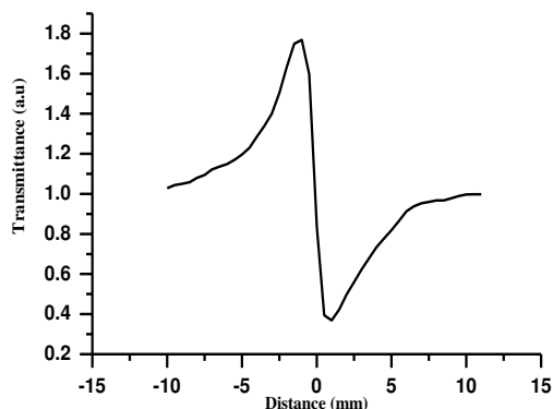
Figure 9. Closed aperture curve of DKFD crystal
