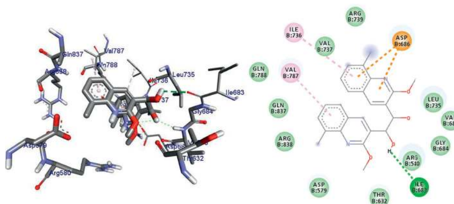
FIGURE 6: The binding interactions of compound 24 against E.coli DNA gyrase A (PDB ID: 1ZIO).
