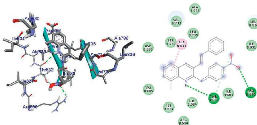
FIGURE 5: The binding interactions of compound 19 against E.coli DNA gyrase A (PDB ID: 1ZIO).
