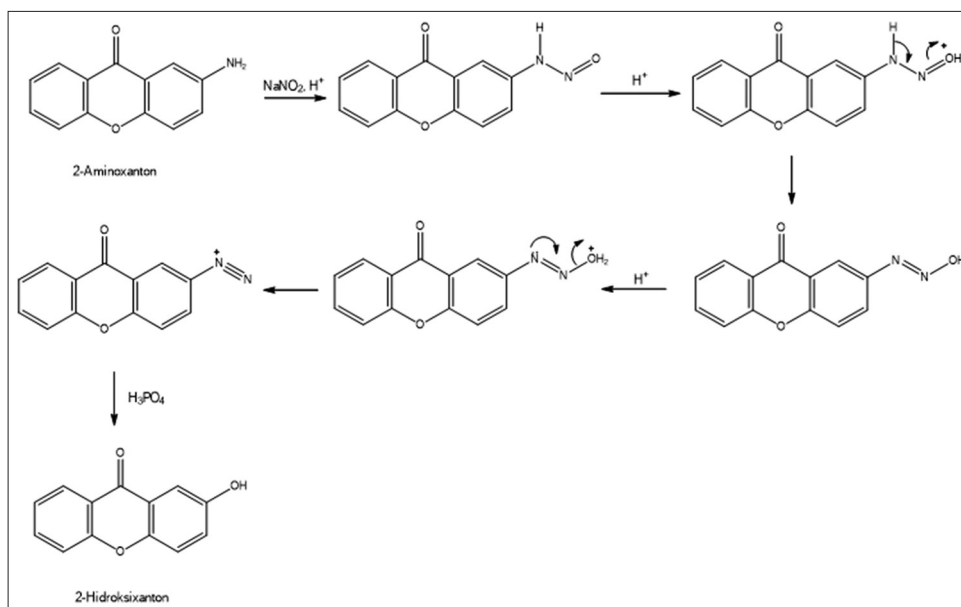
Fig. 4: Mechanism of synthesis of 2-hydroxyxanthone
