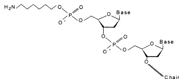
Fig. 1. Oligonucleotide modified in the 5'-position with hexylamine.
