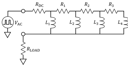
Fig. 15. Test circuit 2 for transient analysis ( V_{AC} = -10 to 10 V, period = 10 \mu\text{s} , duty = 50 %, R_{LOAD} = 5.0 \Omega )
