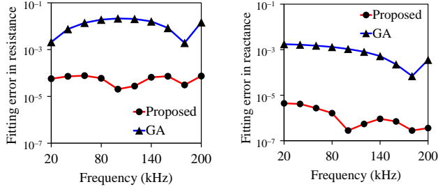
Fig. 5. Fitting errors with 4-stage circuit
