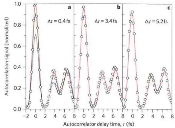
Figure 5 | Sensitivity of the fringe-resolved autocorrelation to \Delta t and \Delta\varphi . a , Central parts of the second-order autocorrelation measured at optimum pulse overlap (black circles) compared to simulations assuming a time delay \Delta t of 0.4 fs and phase offsets of \Delta\varphi = -0.5 rad (red line), 1.1 rad (green line) and 2.6 rad (blue line). b,c , Experimental data and simulations for \Delta\varphi = -0.5 rad, taken at \Delta t = 3.4 fs ( b ) and \Delta t = 5.2 fs ( c ), respectively.
