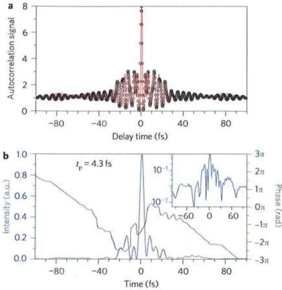
Figure 4 | Characterization of the synthesized single-cycle pulse. a , Second-order autocorrelation trace measured at optimum temporal overlap (red line) and calculated from the combined amplitude and phase spectra in Fig. 2a using a least-square fit varying \Delta t and \Delta\varphi (black circles). b , Temporal intensity envelope (blue lines) and phase (green line) of the combined 4.3-fs light pulse. The inset shows the intensity profile on a logarithmic scale.
