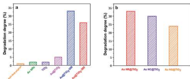
Fig. 4 (a) Photocatalytic degradation of methylene blue by Au NRs, TiO 2 and annealed Au@TiO 2 core-shell nanostructures under visible light. (b) Photocatalytic degradation of methylene blue by Au NR@TiO 2 , Au NC@TiO 2 and Au NS@TiO 2 core-shell nanostructures after annealing under visible light.
