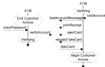
Fig. 11. Derived instances from Fig. 10.
