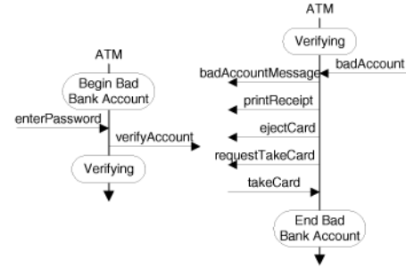
Fig. 10. ATM instance split in two.
