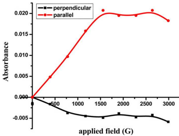
Fig. 6 Field induced optical absorbance for the aqueous ferrofluid in two different polarizations
