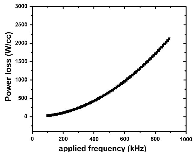
Fig. 7 Power loss spectrum as a function of AC frequency for the ferrofluid
