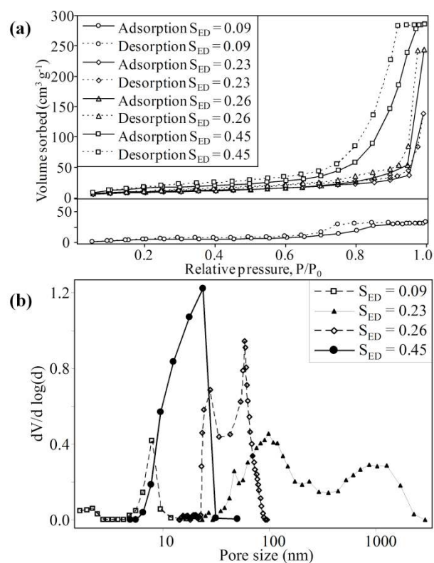
Fig. 5 (a) Nitrogen sorption isotherms of hybrids with various \gamma -PGA:DMSO ratios ( S_{ED} ) and (b) pore size distributions of the same materials obtained from the N 2 desorption isotherm and mercury porosimetry.
