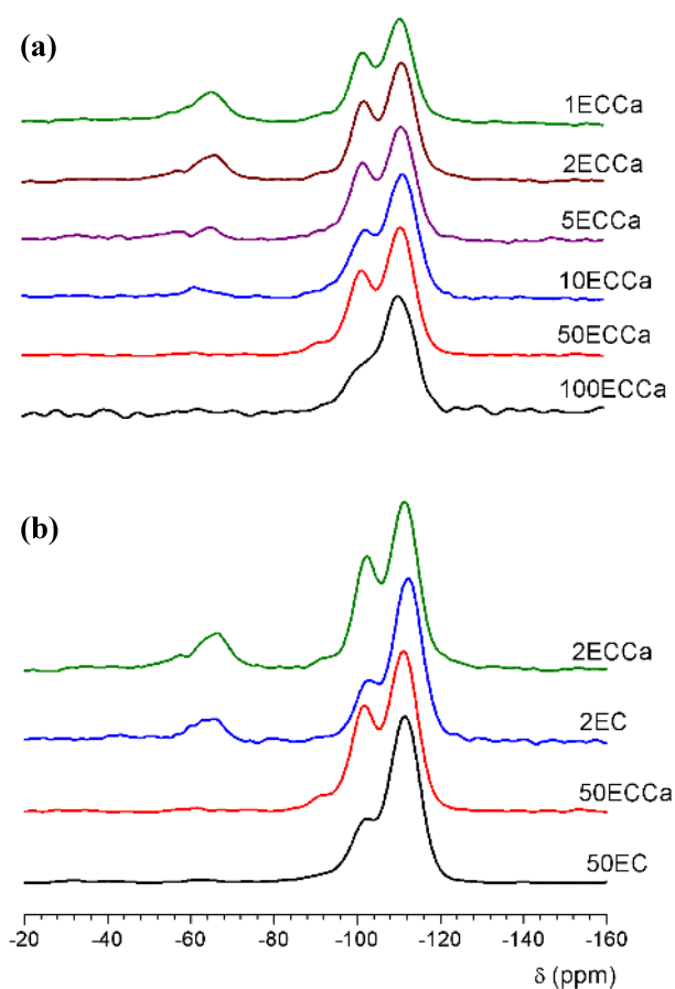
Fig. 8 29 Si MAS NMR spectra of hybrids with increasing amounts of crosslinker (a) and with and without calcium (b).
