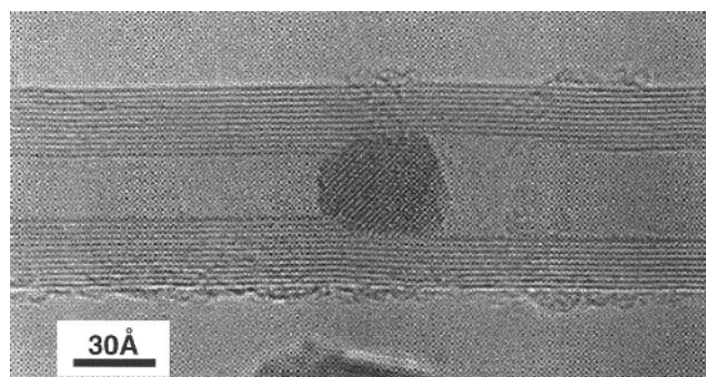
Fig. 2 A high-resolution electron micrograph of an encapsulated \text{FeBiO}_3 crystallite possessing a lattice with a 2.8 Å spacing. This distance corresponds to the inter-layer spacing between the (110) planes of \text{FeBiO}_3 . The crystal appears to have grown where an internal cap is present, as the internal cavity changes diameter at this point.
