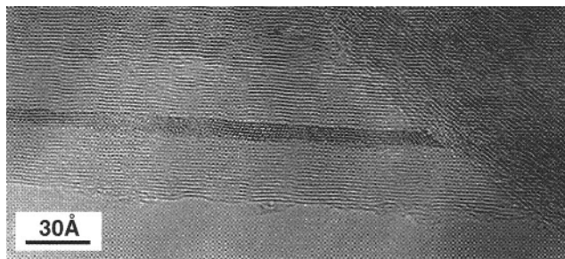
Fig. 3 A high-resolution TEM image of encapsulated polycrystalline ZrO_2 . The observed lattice fringes (1,2) of 2.98 \text{ \AA} correspond to the distance between the (111) planes of the orthorhombic form of ZrO_2 .
