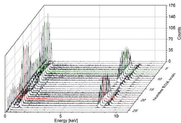
Fig. 6 \gamma - \text{Cu}_3\text{Zn} alloy nanoparticles: HAADF-STEM (top) and local resolution EDX (bottom) of two \gamma - \text{Cu}_3\text{Zn} nanoparticles in [BMIm][BF 4 ] (1.0 wt%). The local resolution EDX scan over two neighboring particles followed the grey line in the TEM; scan width 1 nm, 25 scans show a homogeneous phase of the two \gamma - \text{Cu}_3\text{Zn} nanoparticles; Cu 75.6 \pm 2\% ; Zn 24.4 \pm 2\% (Cu : Zn \approx 3 ). The red and green scan lines indicate the center of each particle.
