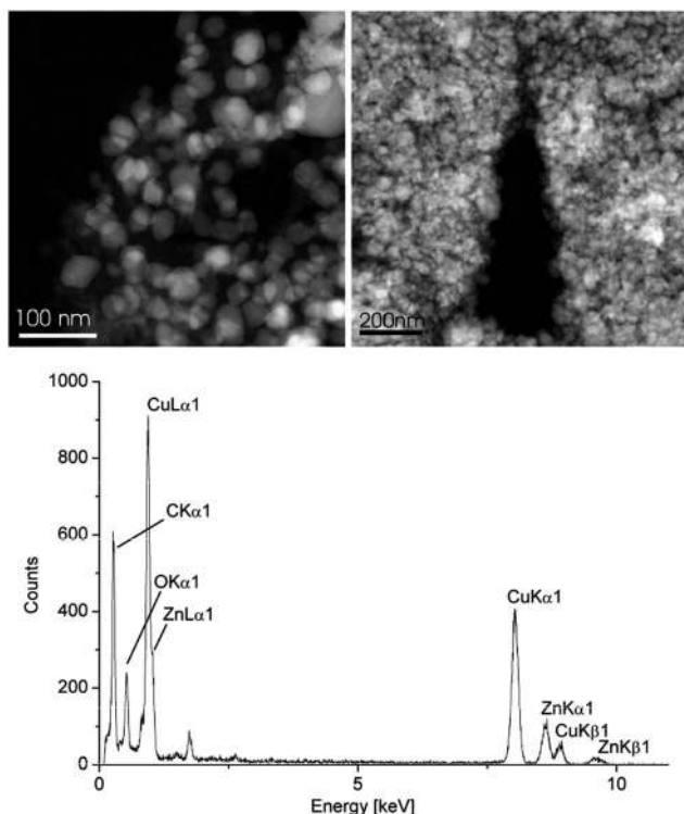
Fig. 5 \gamma - \text{Cu}_3\text{Zn} alloy nanoparticles: HAADF-STEM (top) and EDX (bottom, averaged over 10 particles) of \gamma - \text{Cu}_3\text{Zn} nanoparticles in [BMIm][BF 4 ] (1.0 wt%); Cu 76 \pm 1\% ; Zn 24 \pm 1\% (Cu : Zn \approx 3 ) (minimum estimated errors).
