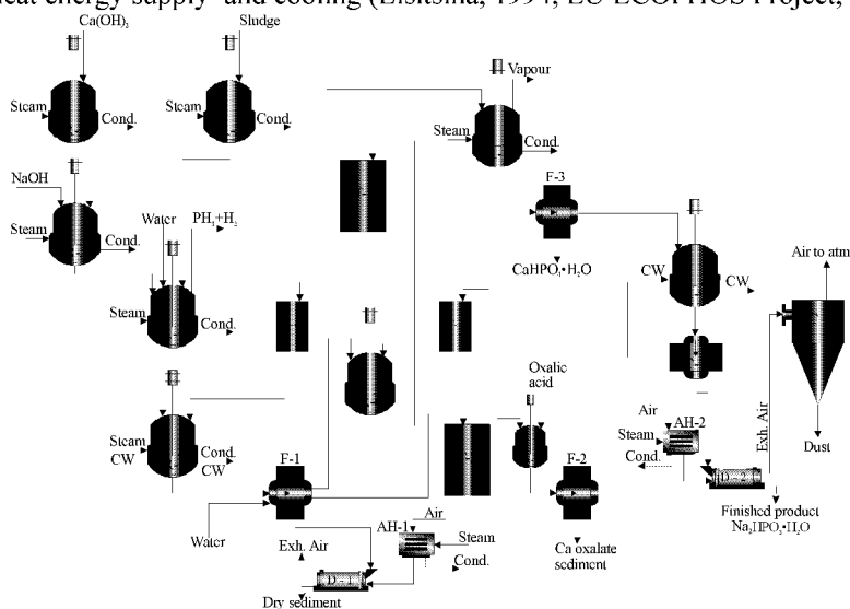
Figure 1. Principal flowsheet for sodium hypophosphite production. R1 - reactor for \text{Ca}(\text{OH})_2 preparation; R2 - reactor for phosphoric sludge preparation; R3 - \text{NaOH}-\text{Ca}(\text{OH})_2 preparation; R4 - main reactor; R5 - following reactor; R6 - neutralization; R7 - evaporator; R8 - sedimentation by oxalic acid; R9 - crystallization; F 1-3 - filter; T 1-4 - tank; C1 - centrifuge; SC1 - cyclone; D 1,2 - dryer; AH 1,2 - air heater.
