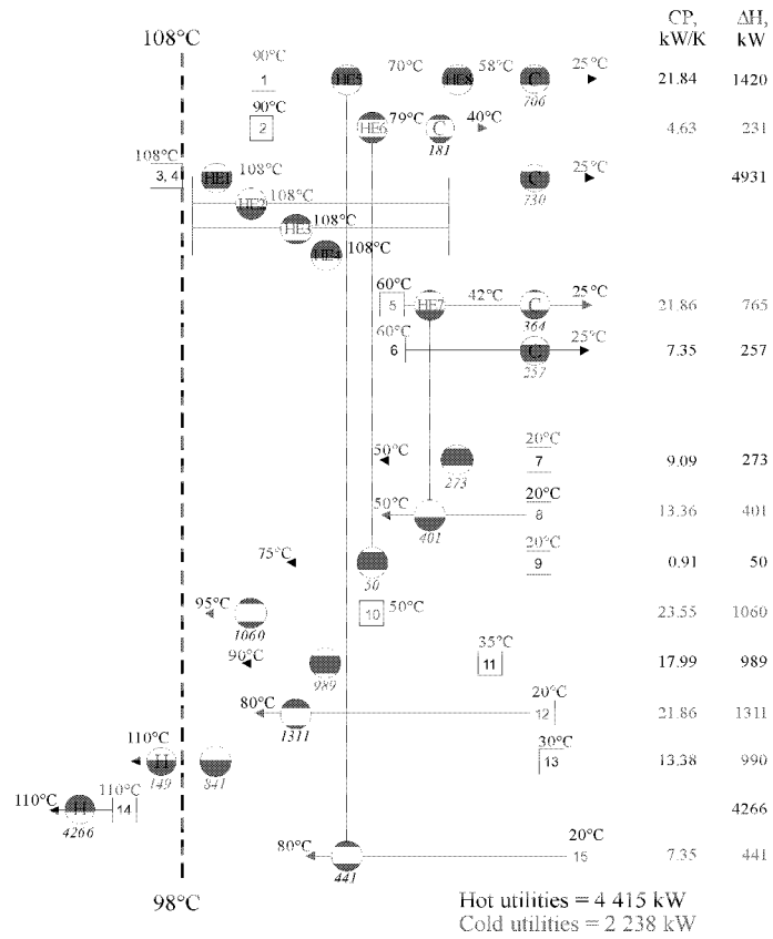
Figure. 4. Grid diagram of integrated process for hypophosphite production with the \Delta T_{min} = 10\text{ }^{\circ}\text{C}
