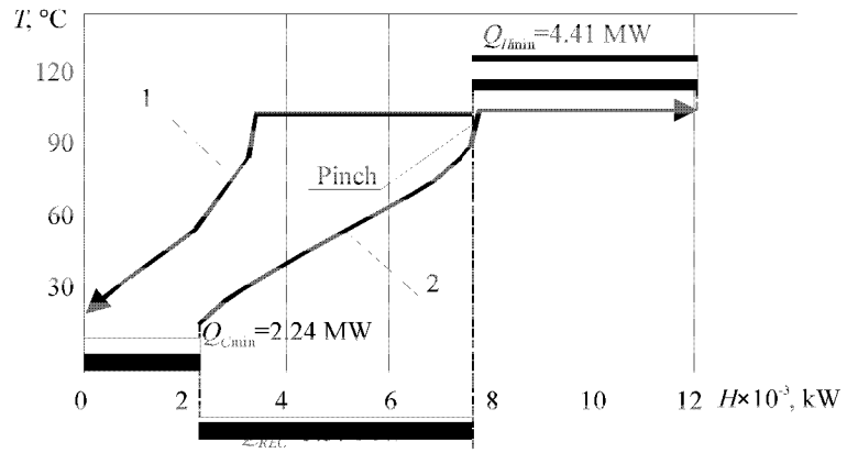
Figure. 3. Composite curves for integrated process at the \Delta T_{min} = 10\text{ }^{\circ}\text{C} : 1– hot composite curve; 2 –cold composite curve. Q_{Hmin} – hot utility; Q_{Cmin} – cold utility; Q_{REC} – recuperation duty
