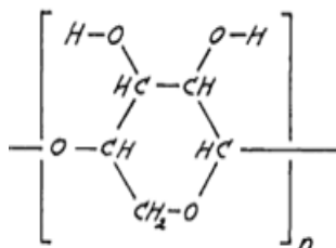
Figure 2.5 Structure of Pentosan
