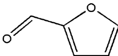
Figure 2.3 Structure of Furfural
