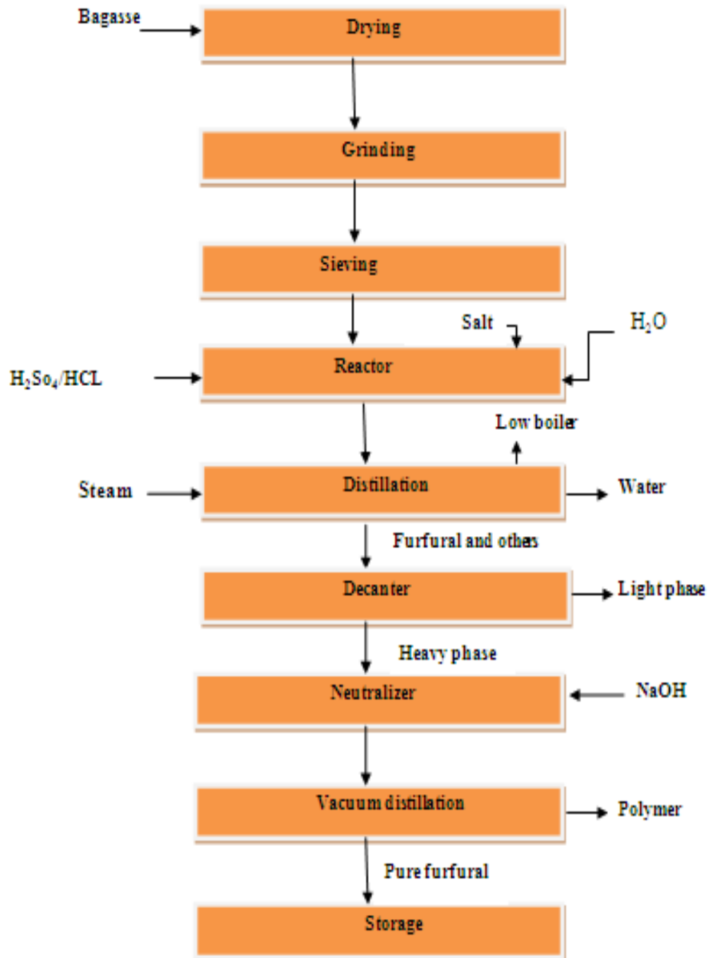
Figure 2.6 Block diagram of furfural production process
