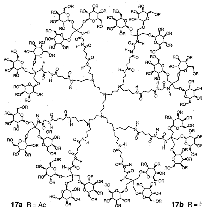
Figure 6. The structure of acetylated trisgalactosidodendrimers 16a and 17a synthesized by attachment (Scheme 3) of active ester 15 to the (DAB)-dendr-(NH 2 ) x dendrimers 1a (top) and 2a (bottom) followed by deacetylation according to Scheme 2.
