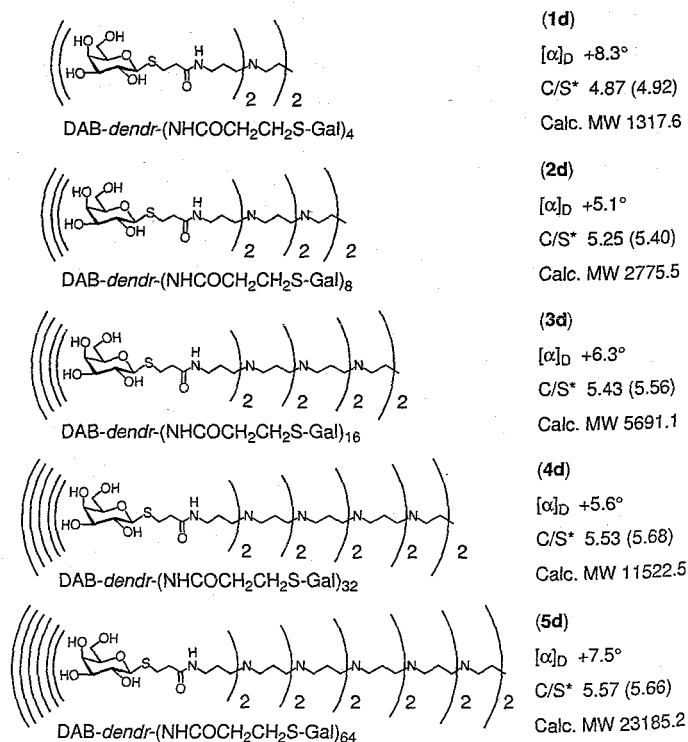
Figure 2. Galactodendrimers 1d–5d . C/S* gives the calculated (and found) microanalyses.
