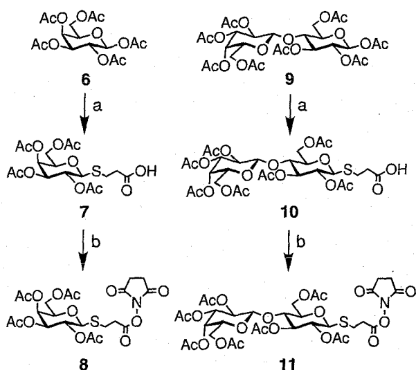
Scheme 1. Synthesis of galactose and lactose derivatives for attachment to the DAB-dendr-(NH 2 ) x dendrimers. Reagents and conditions: a) HS(CH 2 ) 2 CO 2 H/BF 3 ·OEt 2 /CH 2 Cl 2 , 25 °C, 4–5 h, 88% ( 7 ), 53% ( 10 ); b) NHS/DCC/MeO(CH 2 ) 2 OMe, 0–10 °C, 20 h, 93% ( 8 ), 95% ( 11 ).
