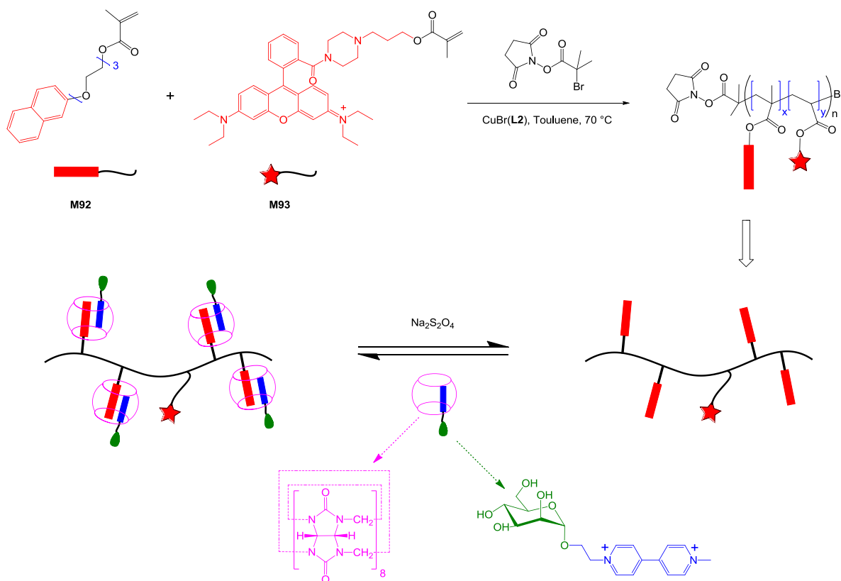
Scheme 19. Post-modification route described by Richards et al. [144] for the synthesis of glycopolymers.
