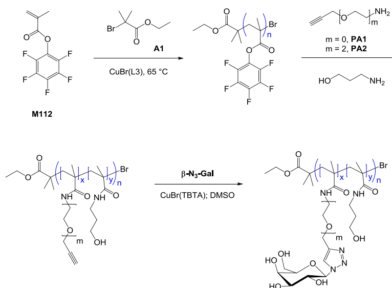
Scheme 19. Post-modification route described by Richards et al. [144] for the synthesis of glycopolymers.
