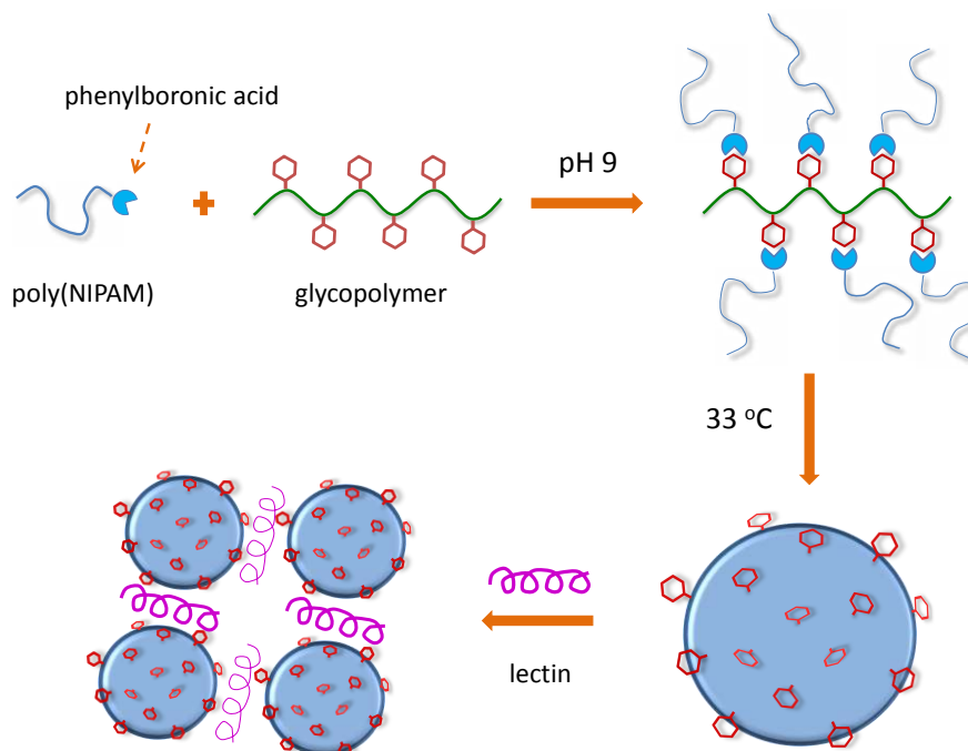
Scheme 22. Synthesis of carbohydrate-decorated polymersomes and their lectin-induced aggregation as reported by Jiang et al. [159].
