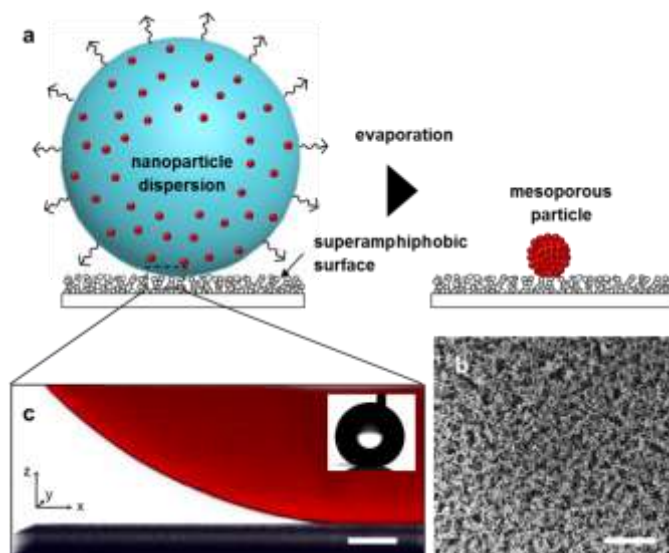
Figure 1. Drop of an aqueous nanoparticle dispersion on a soot-templated superamphiphobic surface. a) A schematic illustration of mesoporous supraparticle formation on the superamphiphobic surface. Due to the high liquid repellency, the shape of the evaporating drop remains spherical throughout the process. b) Scanning electron microscope (SEM) image of the highly porous structure of a superamphiphobic surface prepared by the soot deposition method [10] (scale bar: 10 \mu\text{m} ). c) Interface between the drop and superamphiphobic surface imaged by confocal microscopy. Water (red) was fluorescently labeled with the Alexa488 dye for illustration. Reflection (gray) shows the porous superamphiphobic surface and the drop-air interface (scale bar: 50 \mu\text{m} ). The inset is a side-view of the drop of the nanoparticle dispersion.
