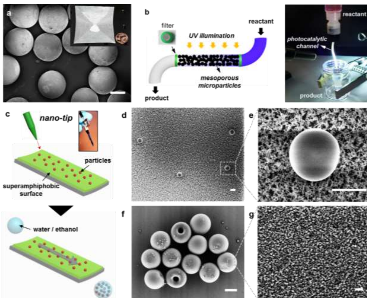
Figure 4. a) TiO 2 mesoporous supraparticles were produced from TiO 2 nanoparticle dispersions (0.1 vol%) dispensed by a fine micropipette (10 μL) and imaged by SEM. The inset shows produced particles as powder. b) A schematic illustration and picture of a tubular photocatalytic reactor for a continuous reaction. The tubular reactor was fabricated with mesoporous TiO 2 supraparticles filled in a 0.8 mm diameter polytetrafluoroethylene tube with 2 μm pore stainless filters. Rhodamine B dye in water was decomposed continuously on the mesoporous TiO 2 particles under UV irradiation. c) A schematic illustration of the multiple particle production process on the superamphiphobic surface with a multi-nanodroplet-dispenser (Nano-Plotter). d), e) The mesoporous TiO 2 particles on the superamphiphobic surface were characterized by SEM. The TiO 2 NP (diameter 7 \pm 2 nm) dispersion droplets were dispensed with a Nano-Plotter and transformed to mesoporous particles after water evaporation in few seconds. f), g) The mesoporous particles were collected by a water/ethanol (1:1 weight) mixture solution and characterized by SEM. The scale bars are 200 μm in a), 10 μm in d) - f) and 100 nm in g).
