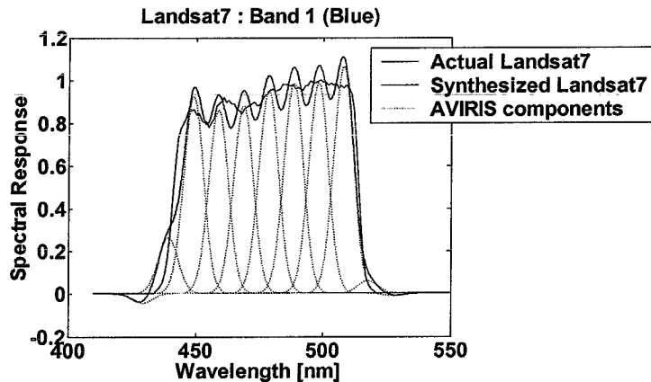
Figure 1. Comparison of actual and simulated spectral response of Landsat 7 ETM+ band 1: hyperspectral components used in the band synthesis are shown as dotted lines.
