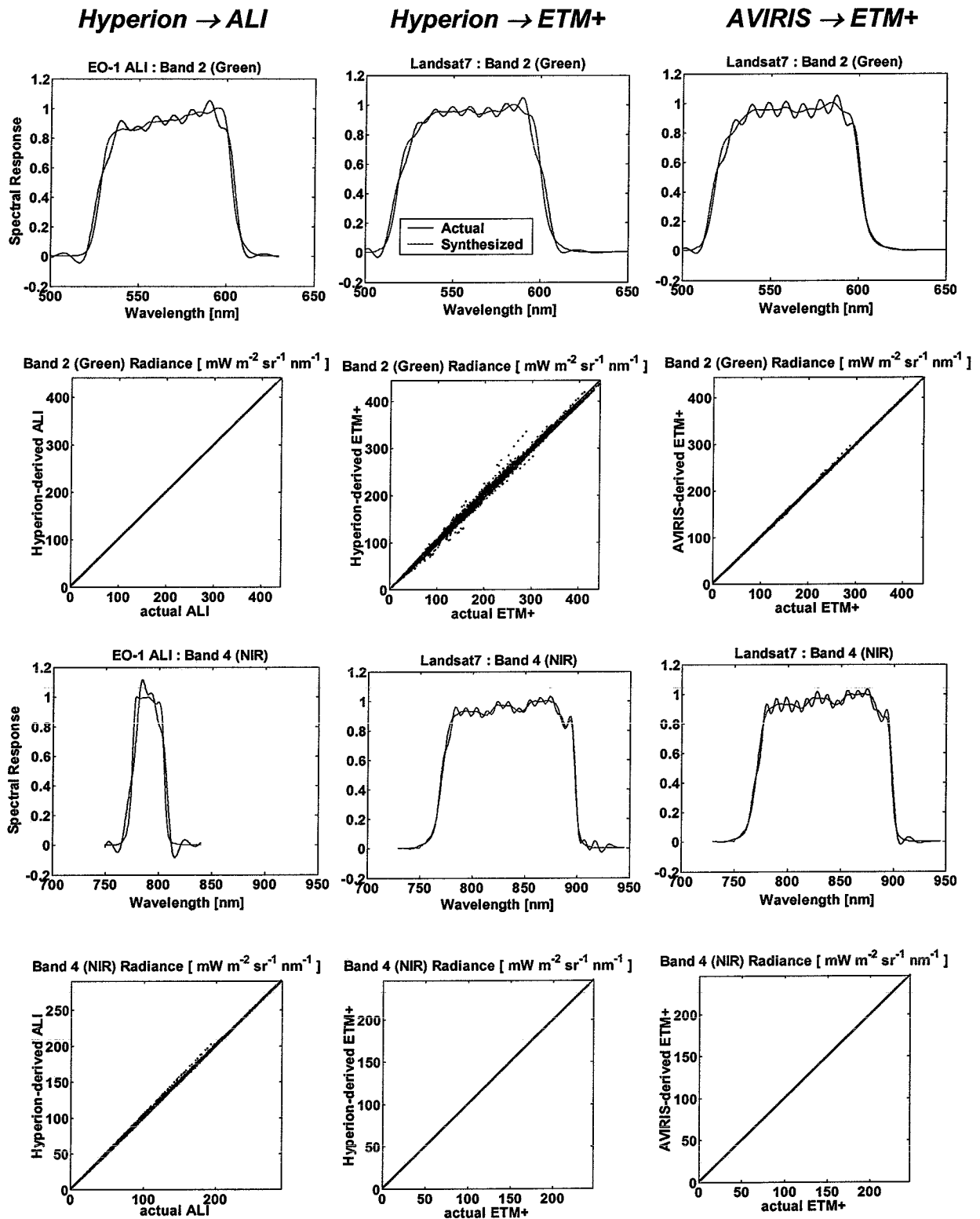
Figure 2. Comparison of spectral band synthesis results and actual spectral responses for band 2 (top row of the upper panel) and band 4 (top row of the lower panel) of the ALI and ETM+ instruments. Scatter plots created from the MODTRAN-generated data (bottom rows of both panels) show moderate effects of the band synthesis artifacts on the simulated images.
