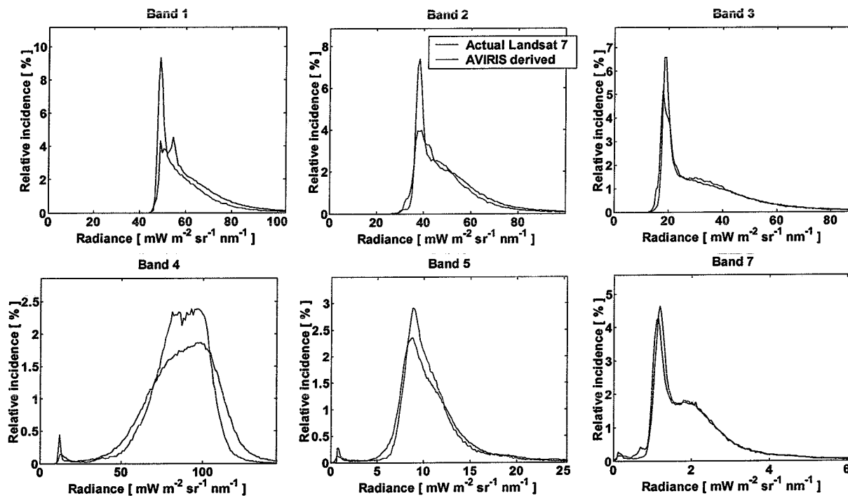
Figure 4. Histograms of radiance values for the actual Landsat 7 ETM+ image and for the image simulated by spectral band synthesis from the AVIRIS hyperspectral data.
