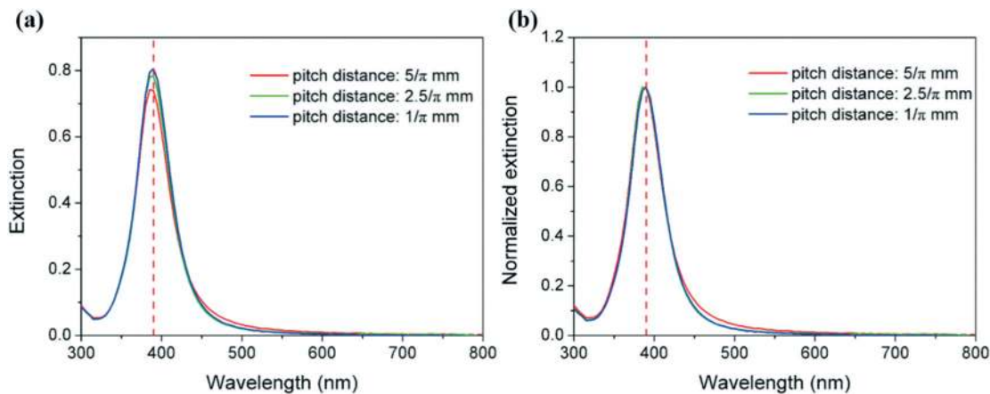
Fig. 13 (a) UV-vis extinction spectra and (b) normalized extinction spectra for AgNPs synthesized in helical tubular microreactors with different pitch distances. Conditions: reactor length: 60 cm, helix diameter: 14 mm, and total flow rate: 0.7 \text{ mL min}^{-1} with an \text{AgNO}_3/\text{NaBH}_4 molar ratio of 1:6.
