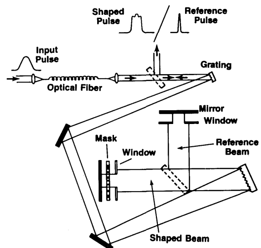
Fig. 1. Experimental apparatus.
