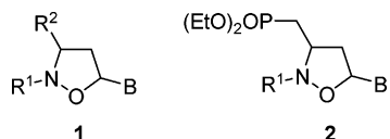
Figure 1. Carbocyclic 2'-oxa-3'-aza-nucleosides.
