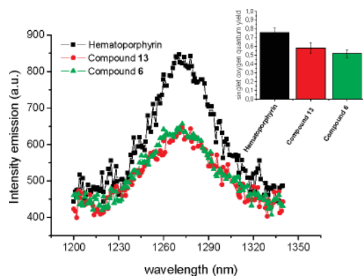
FIGURE 2. Emission spectra of singlet oxygen and singlet oxygen quantum yield ( \Phi_{\Delta} ). Comparison between phthalocyanines 6 and 13 in acetonitrile.
