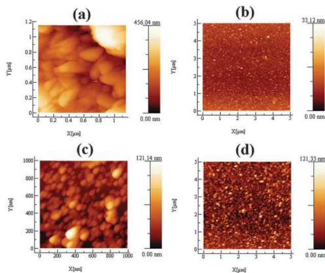
Fig. 13 Height-profile AFM images of transition metal doped pyrite ( \text{M}_x\text{Fe}_{1-x}\text{S}_2 ) thin films deposited at 350 °C on glass substrates by AACVD from complexes (a) (1) and (2), (b) (1) and (3), (c, d) (1) and (5).
