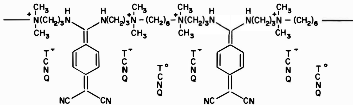
Figure 34: Insertion of TCNQ ° Between Adjacent TCNQ •- .
