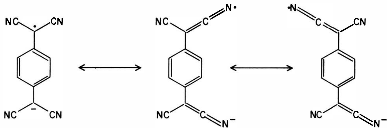
Figure 2: Representative Resonance Forms of TCNQ \cdot^- .
