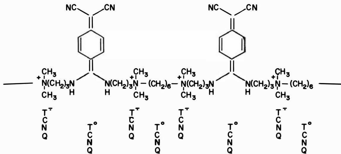
Figure 35: TCNQ Moieties Displaced from Conducting Stacks of the TCNQ 3-6 Polymer by Second TCNQ 0 .
