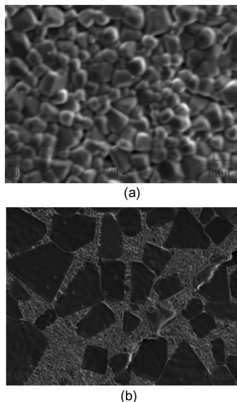
Figure 4. SEM images of CCTO made at 800 °C for 2 h by the combustion method, sintering for 4 h at 1030 °C (a) and 1040 °C (b).
