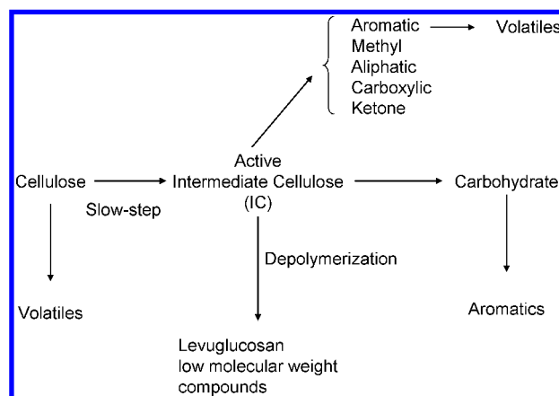
Figure 18. Mechanism for cellulose decomposition adapted from Wooten, Seeman and Hajaligol. 199
