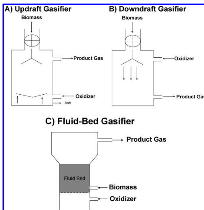
Figure 6. Gasification reactors.
