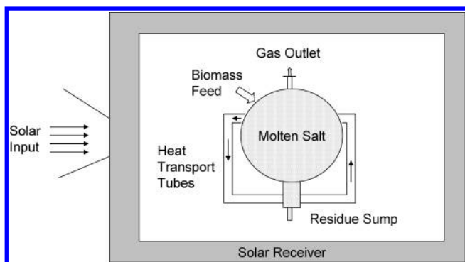
Figure 7. Solar gasification reactor concept. (Figure adapted from Adinberg et al. 84 )
