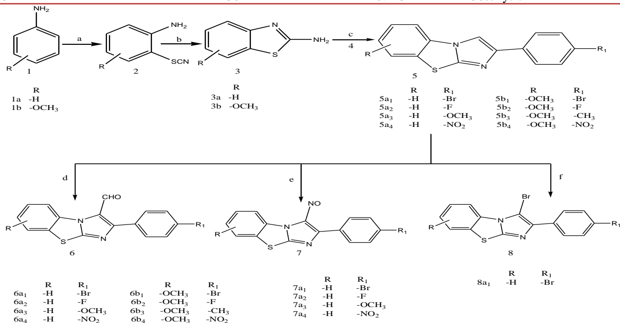
Figure 1: Scheme for the synthesis of 2,3-disubstituted imidazo [2, 1-b] benzthiazole derivatives
