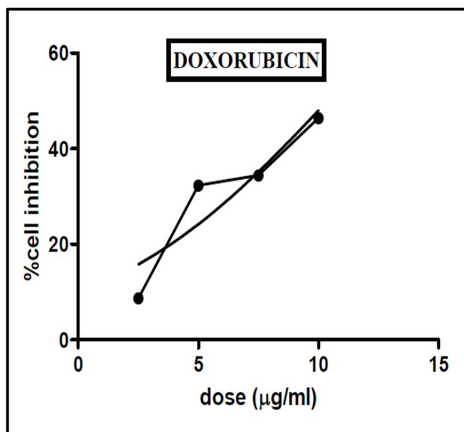
Figure 2: Variation of cell inhibition (%) vs dose (µg/ml) for Doxorubicin
