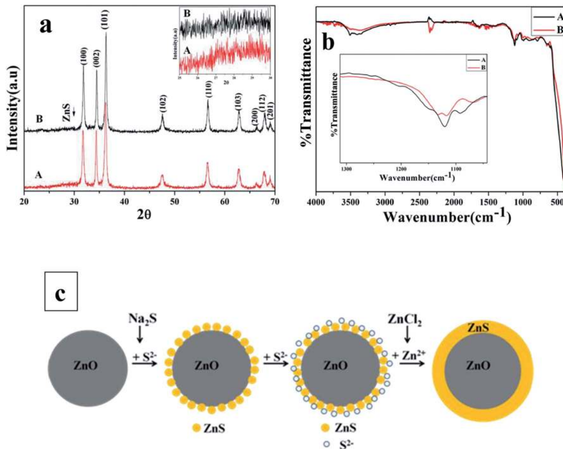
Fig. 7 (a) XRD spectra of ZnO@ZnS CSNPs prepared (a) without and (b) with adding \text{ZnCl}_2 . (b) ATR-FTIR spectra, and (c) A schematic illustration of the ZnO@ZnS CSNPs formation mechanism.
