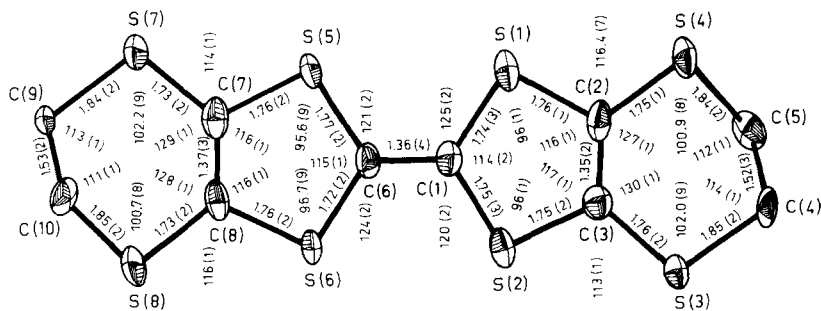
FIGURE 1 BEDT-TTF molecule (A) with bond distances (Å) and angles ( ^\circ ). Thermal ellipsoids at the 50% probability level.
